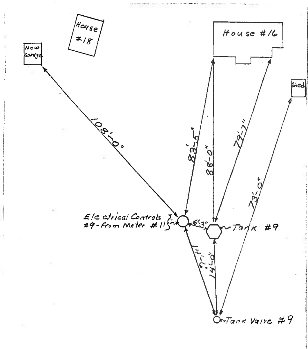
SKETCH J TANK #9 - SERVES HOUSES #16 & #18
