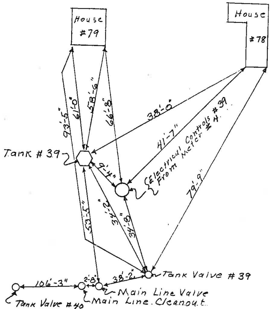
SKETCH 00 TANK #39 - SERVES HOUSE #79 ONLY.
